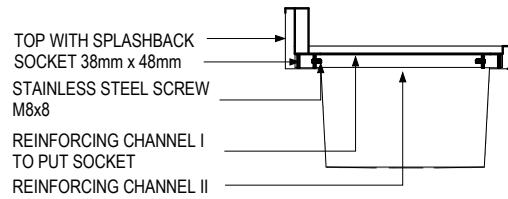
B-SECTION VIEW SCALE 1:15mm
