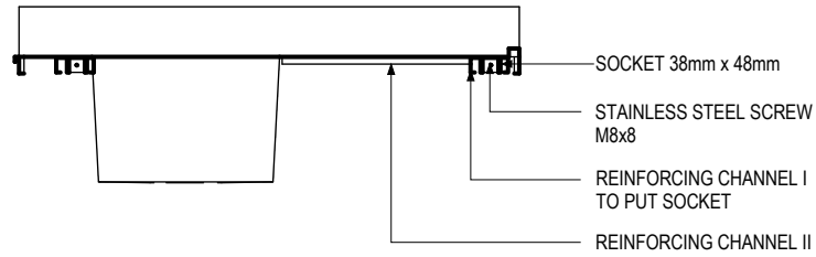
A-SECTION VIEW SCALE 1:15mm
