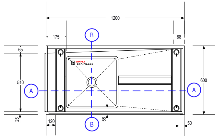
BOTTOM-PLAN VIEW (TOP ONLY)
