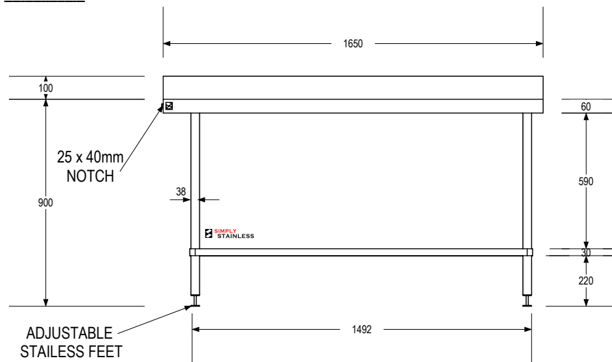
FRONT VIEW
