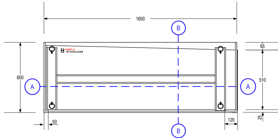
BOTTOM-PLAN VIEW (TOP ONLY)
