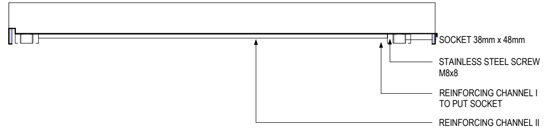
A-SECTION VIEW SCALE 1:15mm
