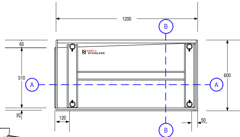
BOTTOM-PLAN VIEW (TOP ONLY)
