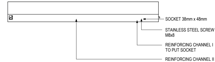
A-SECTION VIEW SCALE 1:15mm
